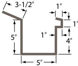
Gutter Hanger
