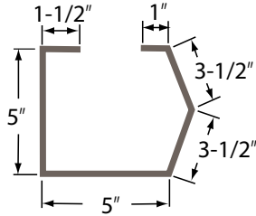
Sculptured Gutter
