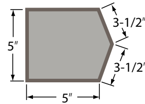
Box Gutter Endcap
