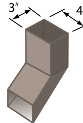
3" X 4" 45° Elbow
